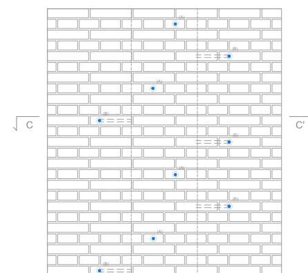
ELEVATION C
