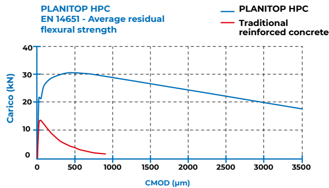
Graph representing residual flexural strength in compliance with EN 14651 standards
