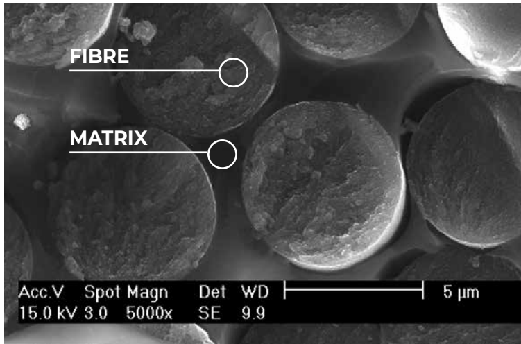
→ An image of FRP composite materials through a microscope.
