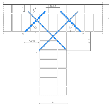
SECTION BB' (internal stitching)
