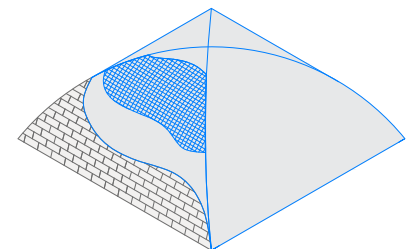
CLOISTER VAULT AXONOMETRY
