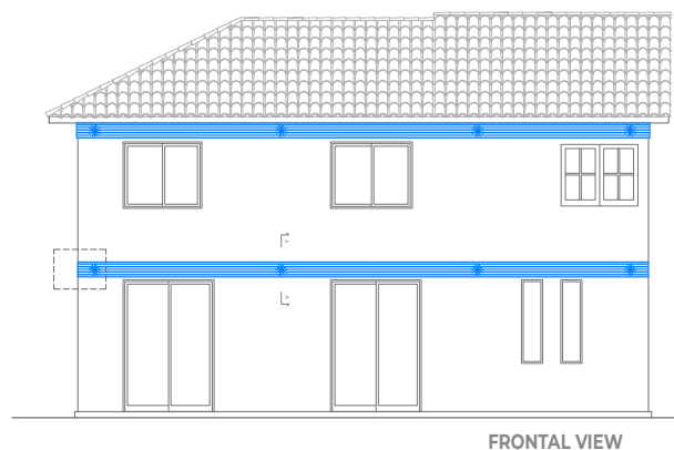
FRONTAL VIEW
