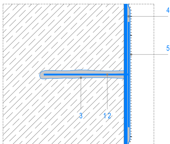
CLOSE-UP VIEW OF A BLIND TIE
