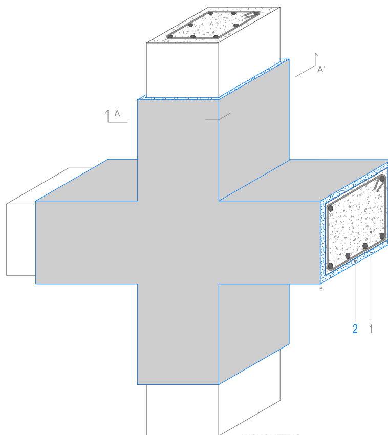
AXONOMETRIC PROJECTION
