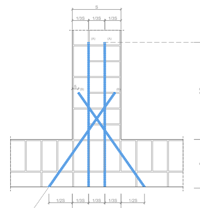
SECTION CC' (external stitching)
