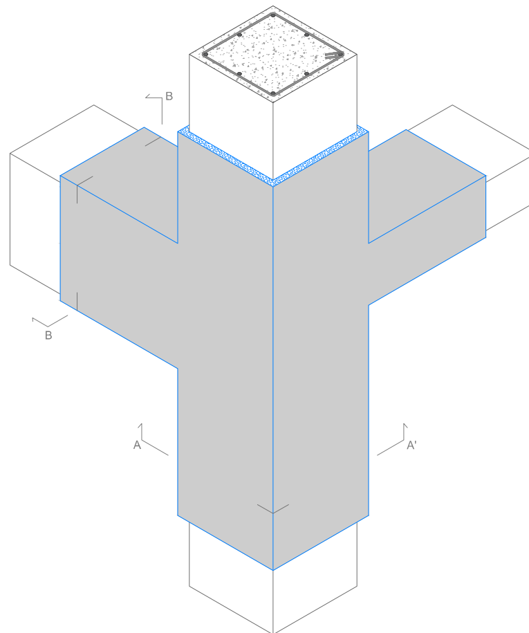
AXONOMETRIC PROJECTION
